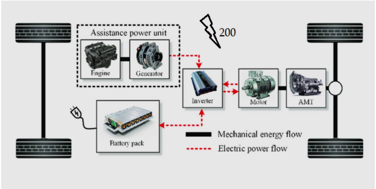
Figure 2: Intelligent Plug-In Hybrid Electric Vehicles Block Diagram.
