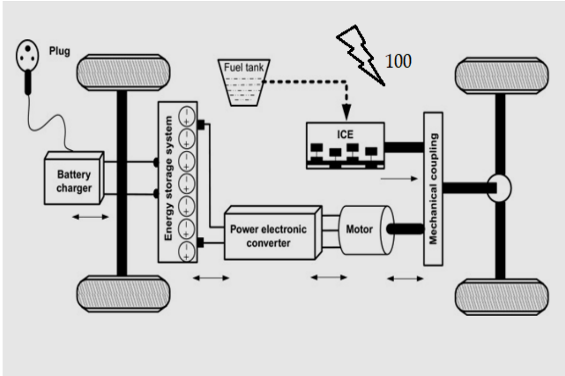
Figure 1: Intelligent Plug-In Hybrid Electric Vehicles Flow Chart.
